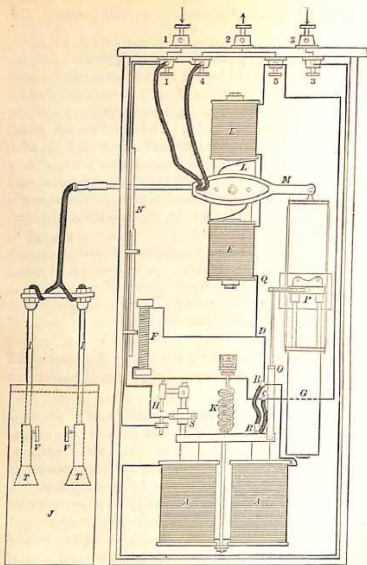
Fig. 47.—Schuyler Regulator.
