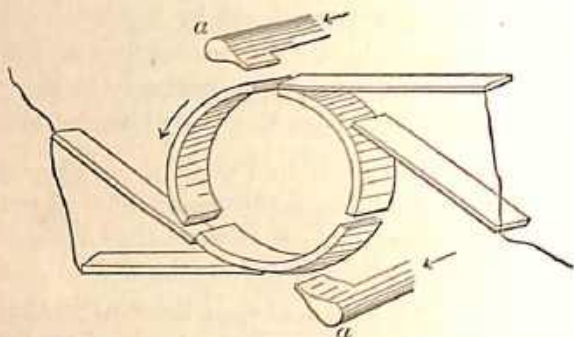
Fig. 23.—Three-Segment Commutator, Brushes and air Blast of Thompson-Houston Arc Dynamo.
