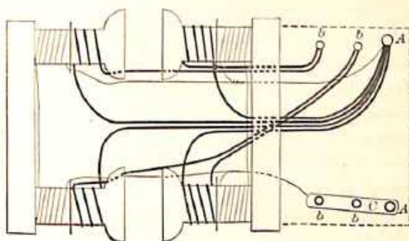
Fig. 36.—Connections of Compound Wound, Automatic Regulating Dynamo.
