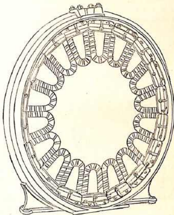
Fig. 5.—Mordey Armature.
