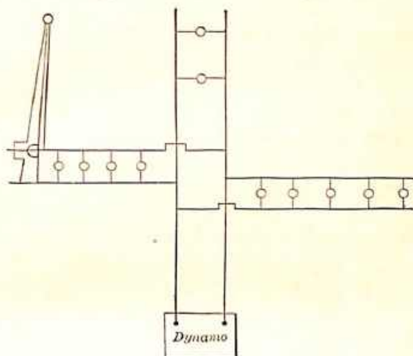
Fig. 8.—Parallel or Multiple Arc System.
