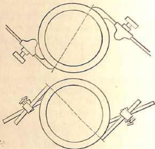
Fig. 26.—Double Brushes.
