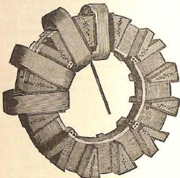
Fig. 32.—Brush Armature.
