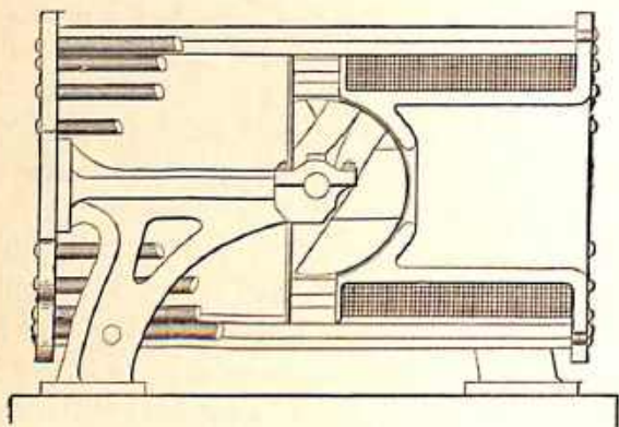
Fig. 48.—Thomson-Houston Dynamo.
