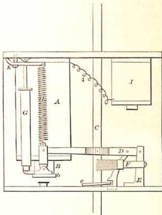
Fig. 19.—Side View of Mechanism of Arc Lamp.
