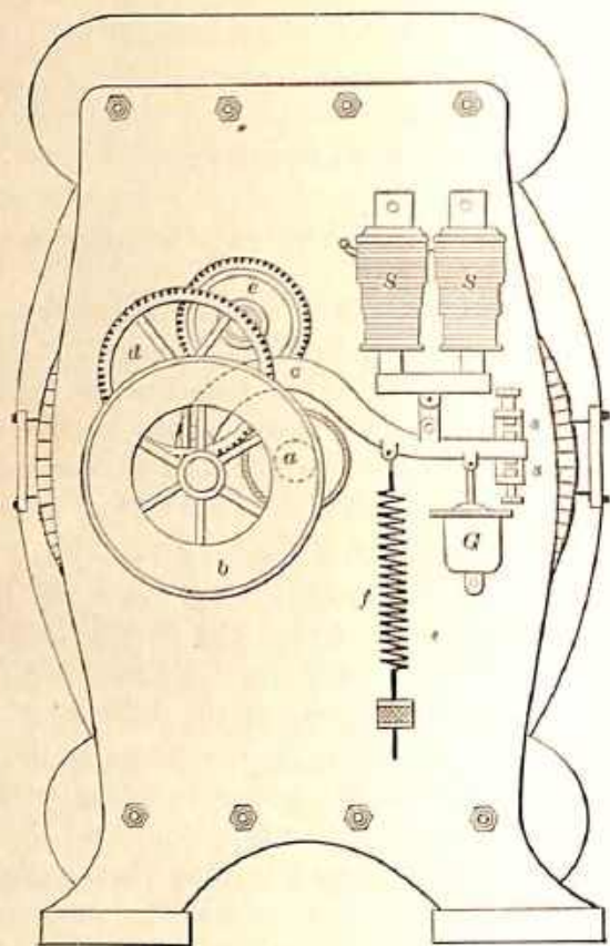
Fig. 31.—Regulator of American System.
