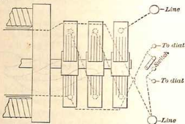
Fig. 35.—Connections of a No. 8 Brush Dynamo.
