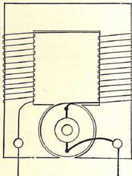
Fig. 78.—Series Winding.
