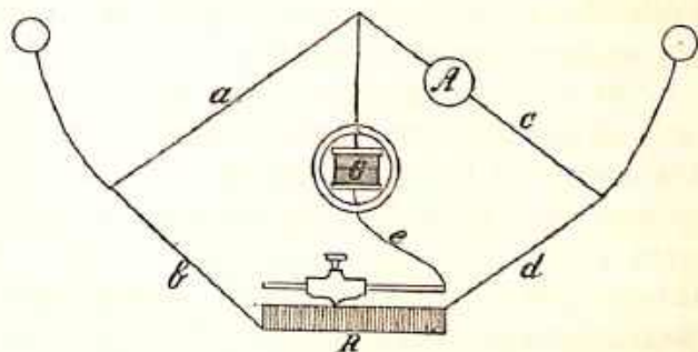
Fig. 41.—Diagram of Circuits of Howell Pressure Regulator.
