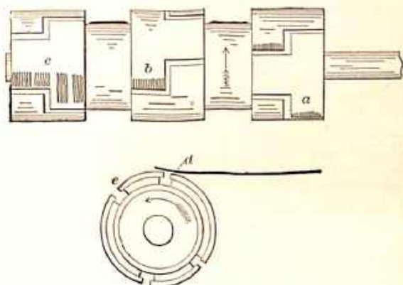
Fig. 2A.—Brush Commutator, Side and End Views.
