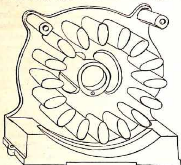
Fig. 8.—Ferranti Field Magnets.
