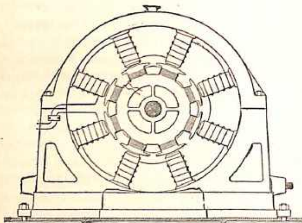
Fig. 10.—Stanley Constant Current Dynamo.
