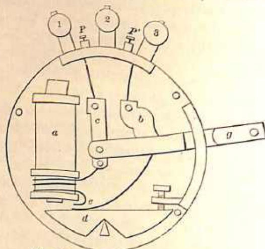
Fig. 12.—Multiple-Series Cut-Out.
