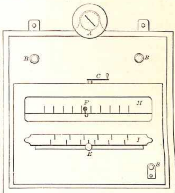
Fig. 40.—Front View Howell Indicator.
