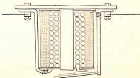
Fig. 10.—Automatic Cut-Off.
