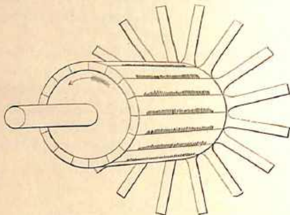
Fig. 22.—Multiple Segment Commutator.
