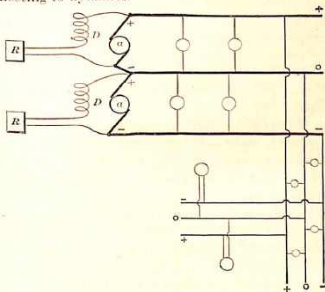
Fig. 15.—Three-Wire System.
