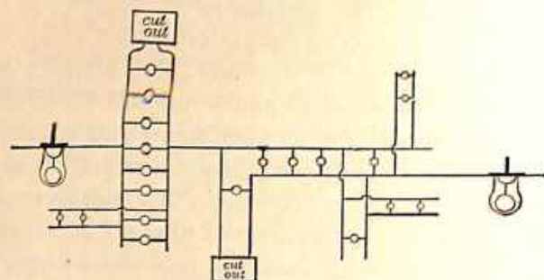
Fig. 11.—Multiple-Series System.
