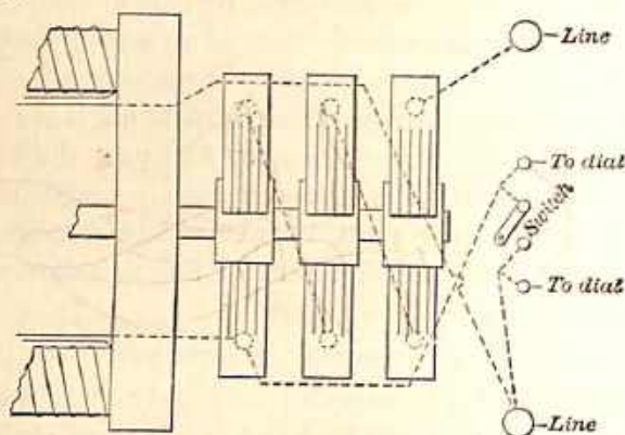
Fig. 35.—Connections of a No. 8 Brush Dynamo.
