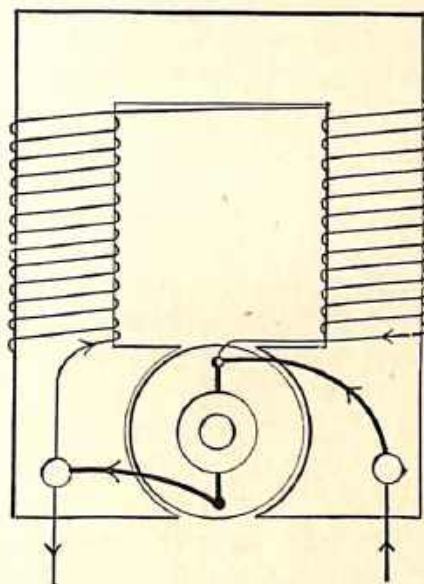
Fig. 79.—Shunt Winding.
