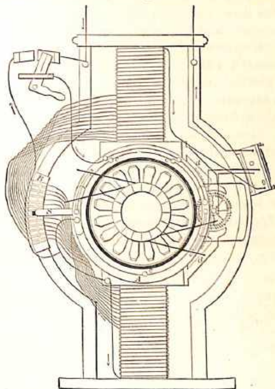
Fig. 42. - Excelsior Dynamo and Regulating Apparatus.
