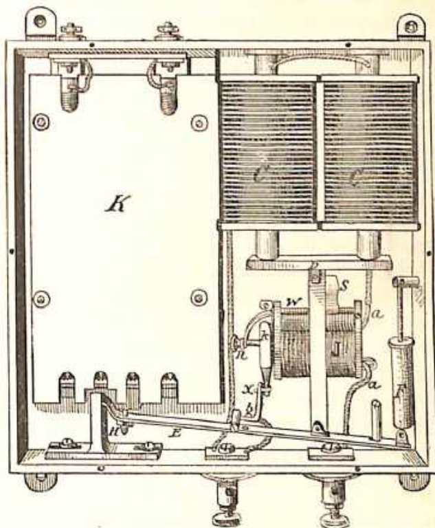
Fig. 34.—Dial Controller.
