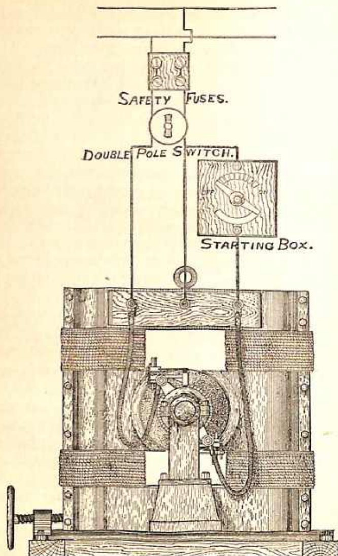
Fig. 80.—Shunt Motor, Connections and Starting Box.
